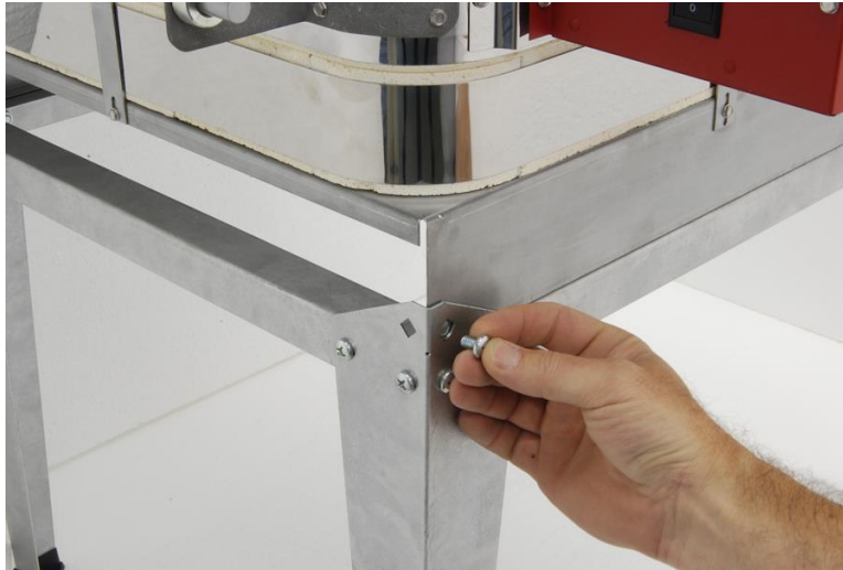
Insert a bolt through each front leg and kiln base and secure with nut.
